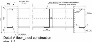
Detail A floor steel construction schaal 1:5
