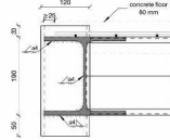
Detail B floor steel construction schaal 1:5
