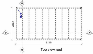
Top view roof
