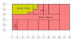
Brandcompartimentering
